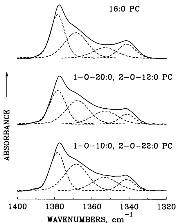
FIGURE 1 The \text{CH}_2 region of the infrared spectra in the liquid-crystalline phases of 16:16 PC (top), 20:12 PC (middle) and 10:22 PC (bottom). The absorbance spectra shown have been corrected for solvent and water vapor absorption, and baseline-corrected by cubic spline interpolation. The solid lines indicate the contours of the absorption bands observed, and the dashed lines indicate estimates of the component bands as derived by a combination of Fourier deconvolution and curve fitting.
