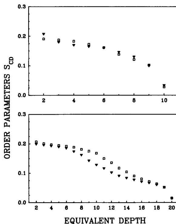
FIGURE 7 Comparison of the ^2\text{H} orientational order profiles of 20:12 PC and 10:22 PC as a function of the equivalent depth of the lipid bilayer. The orientational order profiles of the short chains ( top ) and long chains ( bottom ) are compared at T_m + 6^\circ\text{C} . The filled symbols define the order profiles of 10:22 PC, and the open symbols define the order profiles of 20:12 PC.
