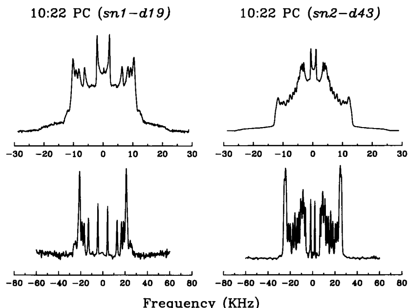
FIGURE 2 ^2\text{H} -NMR spectra of the two chain perdeuterated analogs of 10:22 PC. Data are presented for sn1 - \text{d}_{19} 10:22 PC (left panel, short-chain perdeuterated) and sn2 - \text{d}_{43} 10:22 PC (right panel, long-chain perdeuterated). The spectra recorded are shown in the top panel, and the corresponding "dePaked" spectra shown in the bottom panel.
