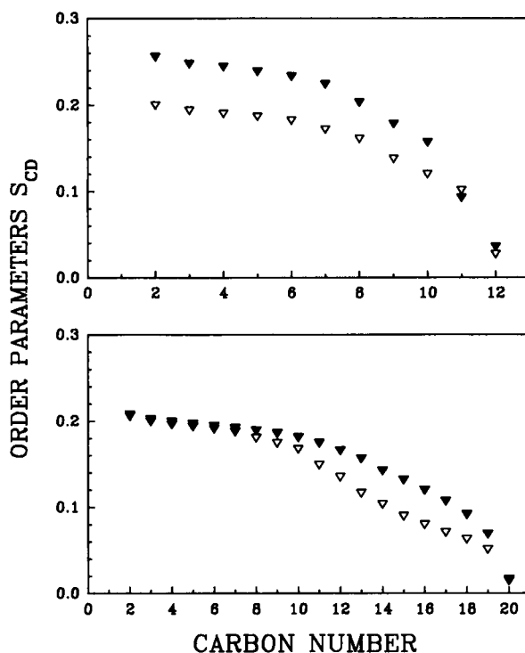
FIGURE 4 Comparison of the ^2\text{H} orientational order profiles of the long and short chains of the asymmetric chain PC with those of long- and short-chain symmetric chain PC. Each of the order profiles shown was derived from spectra acquired at comparable reduced temperatures ( T_m + 6^\circ\text{C} ). The top panel shows the orientational order profiles described by the dodecanoyl chains of 20:12 PC ( \nabla ) and sn 2- \text{d}_{23} 12:12 PC ( \blacktriangledown ). The bottom panel shows the orientational order profiles described by the eicosanoyl chains of 20:12 PC ( \nabla ) and chain-perdeuterated 20:20 PC ( \blacktriangledown ).
