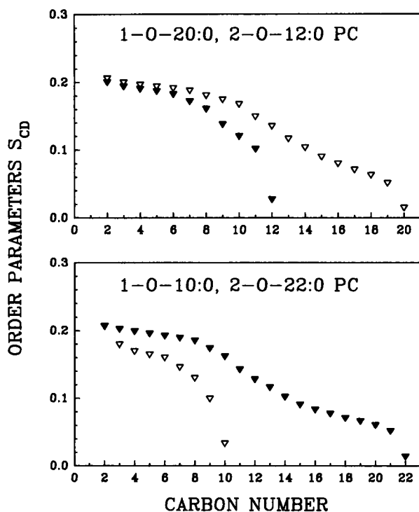
FIGURE 3 ^2\text{H} -NMR order profiles derived from the dePaked spectra of specifically chain-perdeuterated analogs of 10:22 PC ( bottom panel) and 20:12 PC ( top panel) at temperatures just above T_m . The orientational order parameters are plotted as a function of hydrocarbon chain number. The open symbols describe the order profiles obtained from sn 1 chain-perdeuterated lipids, and the filled symbols describe the order parameters obtained from the sn 2 chain-perdeuterated lipids.
