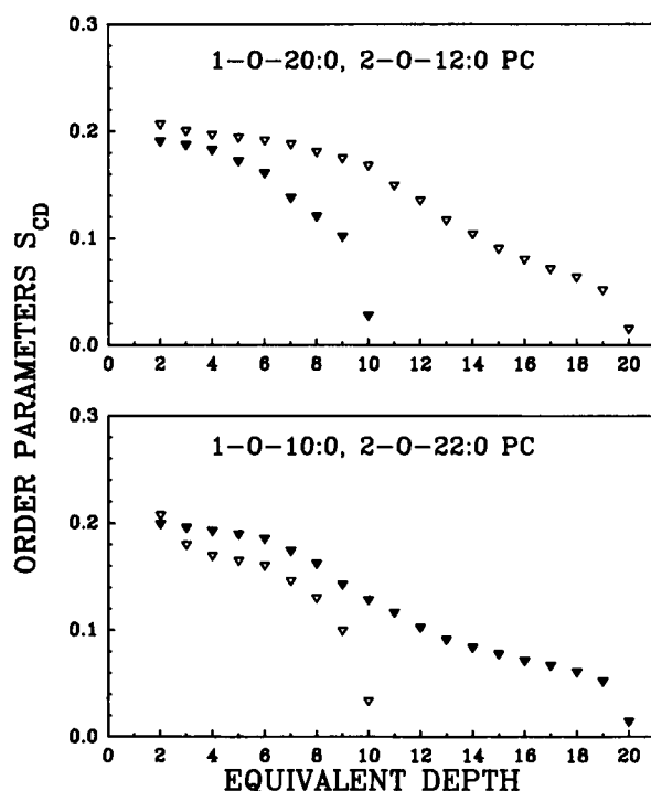
FIGURE 6 Comparison of the ^2\text{H} orientational order profiles described by the long and short chains of 20:12 PC ( top ) and 10:22 PC ( bottom ) as a function of the equivalent depth of the lipid bilayer. The open symbols describe the orientational order profiles of the sn 1 fatty acyl chains, and the closed symbols describe the orientational order profiles of the sn 2 fatty acyl chains. The data shown were all acquired at T_m + 6^\circ\text{C} .
