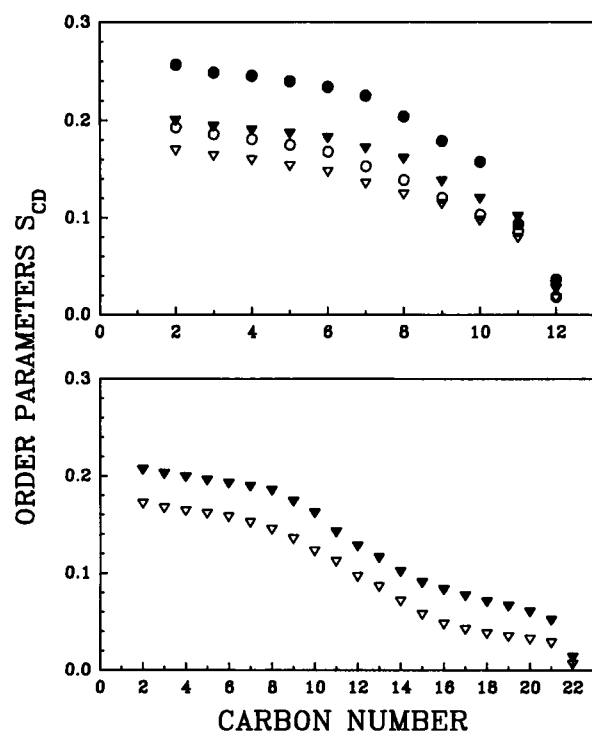
FIGURE 5 Effect of temperature on the ^2\text{H} orientational order profiles of the dodecanoyl chains of sn 2- d_{23} 12:12 PC PC (top, \circ , \bullet ), the dodecanoyl chains of 20:12 PC (top, \nabla , \blacktriangledown ) and the docosanoyl chains of 10:22 PC (bottom). The closed symbols describe order profile obtained from spectra acquired at T_m + 6^\circ\text{C} , whereas the open symbols describe the order profiles obtained from spectra acquired at T_m + 40^\circ\text{C} .
